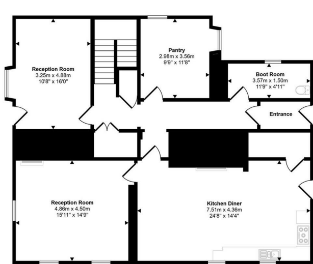
Lower Ground Floor Approx 128 sq m / 1378 sq ft
